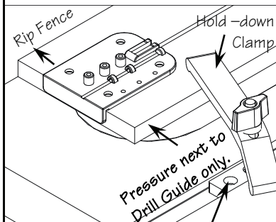
Micro Jig ZeroPlay™ Guide Bar Stop
