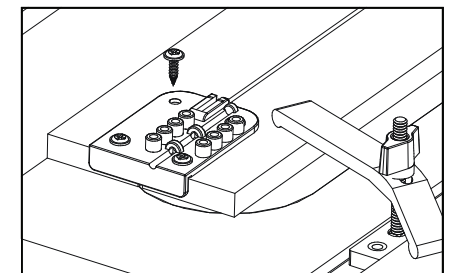
Micro Jig ZeroPlay™ Guide Bar Stop
