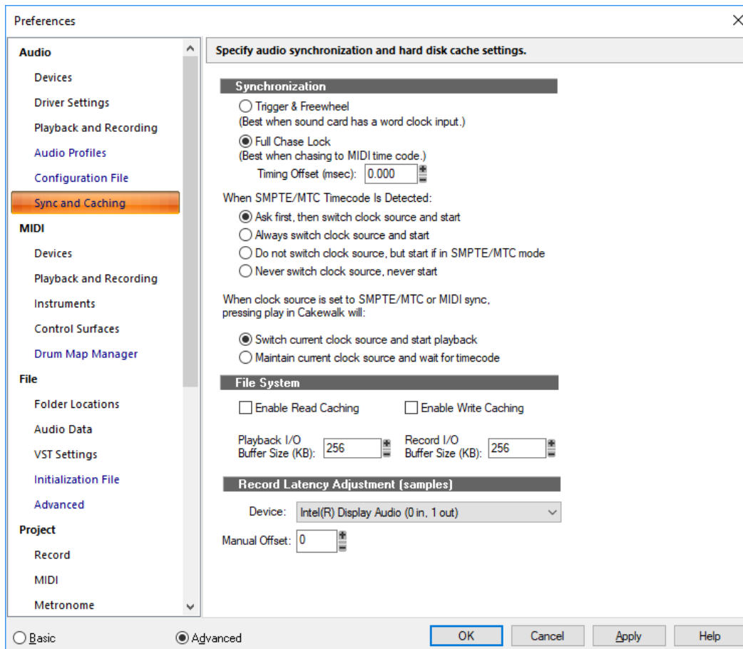
Figure 618. The Sync and Caching section.
