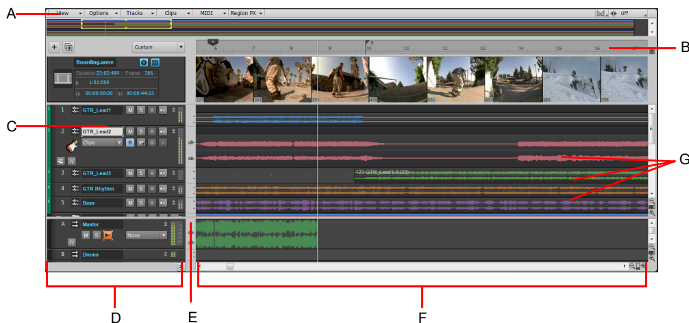
Figure 647. The Track view.
