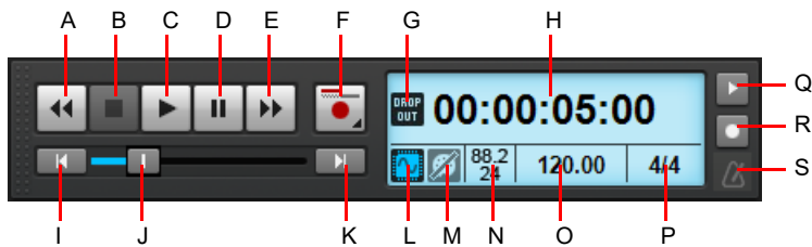
Figure 297. The Transport module.
