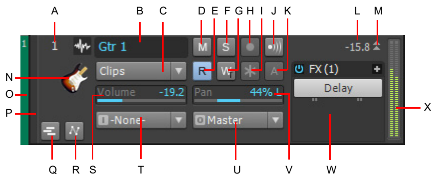
Figure 108. Audio track controls.
