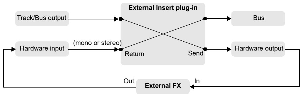
Figure 443. External Insert signal flow.
