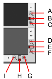
Figure 84. Zoom controls.
