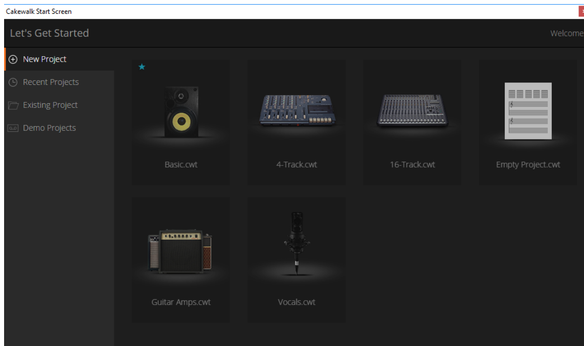
Figure 645. Start Screen.
