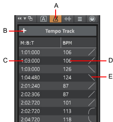
Figure 3. Tempo Inspector.
