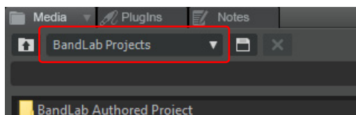
Figure 157. Media Browser.
