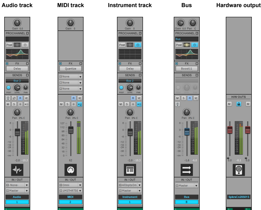
Figure 658. The controls displayed in a channel strip vary according to the channel strip type.
